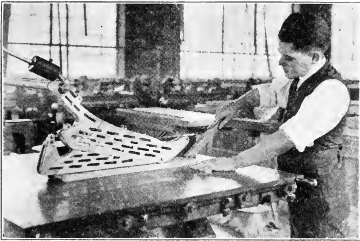
FIG. 160. RIPPING NARROW STOCK.
